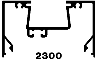
2300 OPEN BACK MULLION
