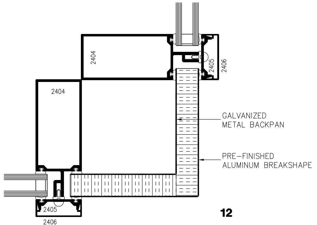
90° BREAKSHAPE CORNER
