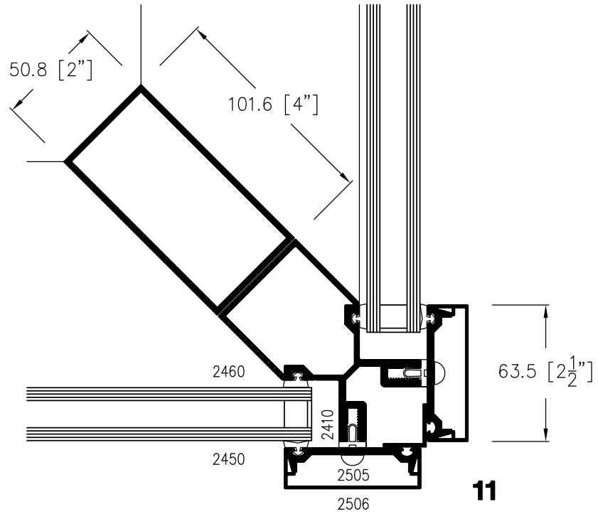
90° CAPTURED CORNER
