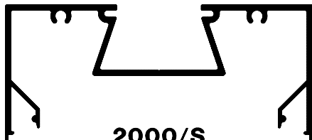
2000/S OPEN BACK MULLION/ SHALLOW POCKET
