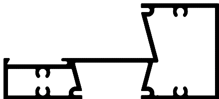
2016 TUBULAR SILL/ HORIZONTAL MULLION
