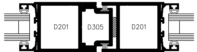
5 OXOXO MEETING STILE
