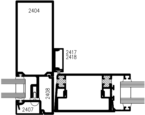
SWING DOORS
