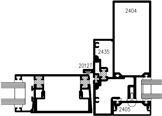
SWING DOORS
